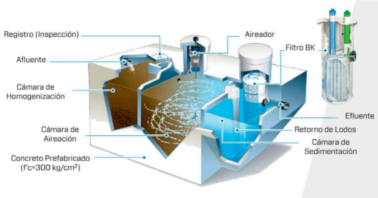
Figure 5. PTAR Singular
