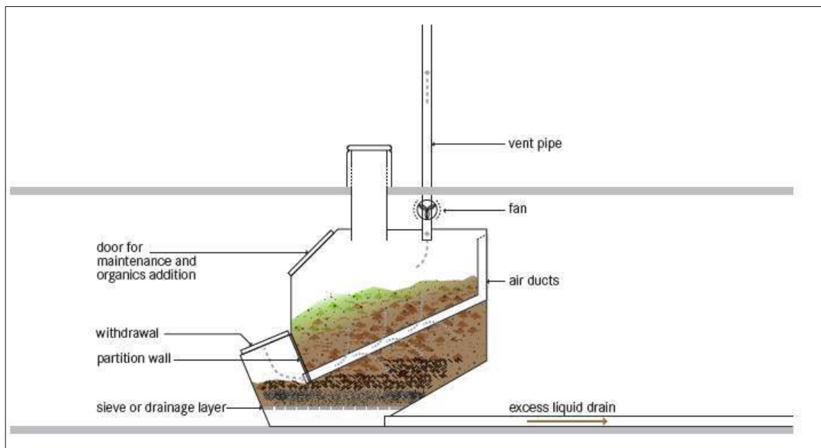
Figure 6. Composting chamber.
